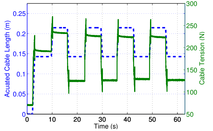
Fig. 8: Motor mount torque sensor data and motor position data recorded during a square wave input position trajectory for a single motor. This plot shows measured tension from the sensor and cable length from motor encoder measurements as a function of time for this dynamic movement.
