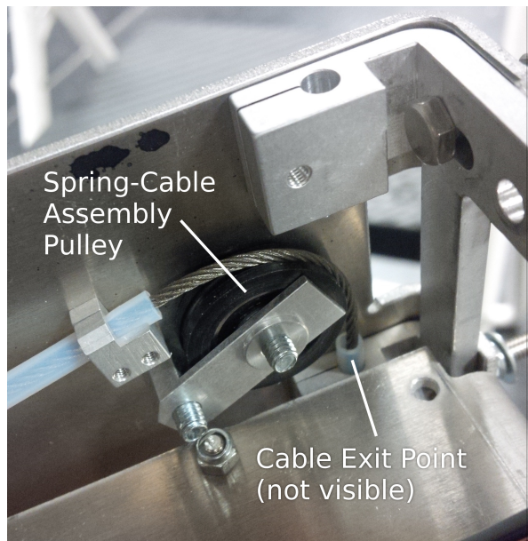
Fig. 5: Internal view of the pulley and exit point of the steel cable, which connects to springs inside the strut tube on one end and to the external vectran cables on the other.
