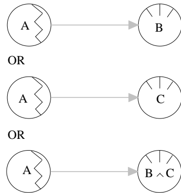
Fig. 16. Alternative representation for rule: IF A THEN B OR C
