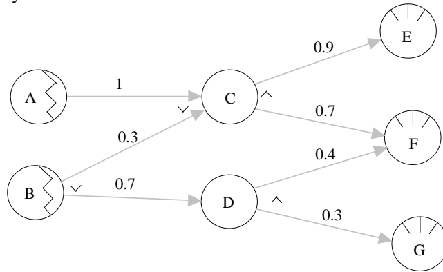
Fig. 17. Fuzzy belief net: illustrative example
