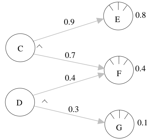
Fig. 17: Operations to solve fuzzy influence diagram; example case
