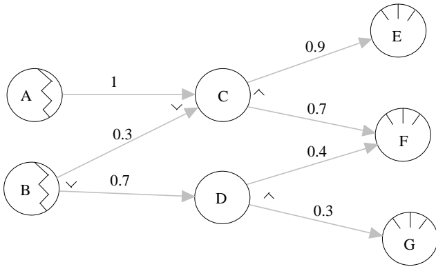
Fig. 16: Fuzzy belief net: illustrative example
