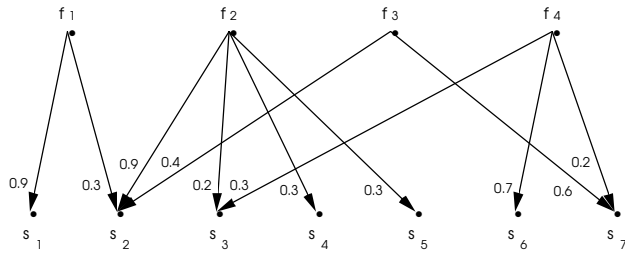
Fig. 1: Fuzzy causal diagram
