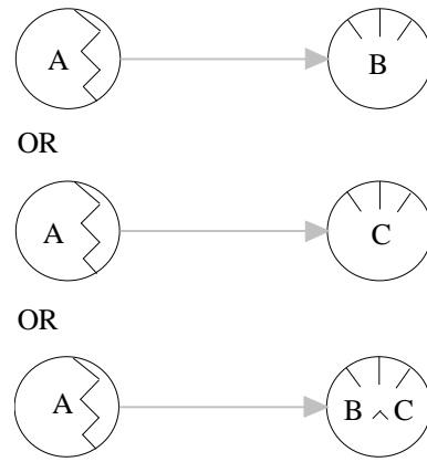
Fig. 15: Alternative representation for rule: IF A THEN B OR C
