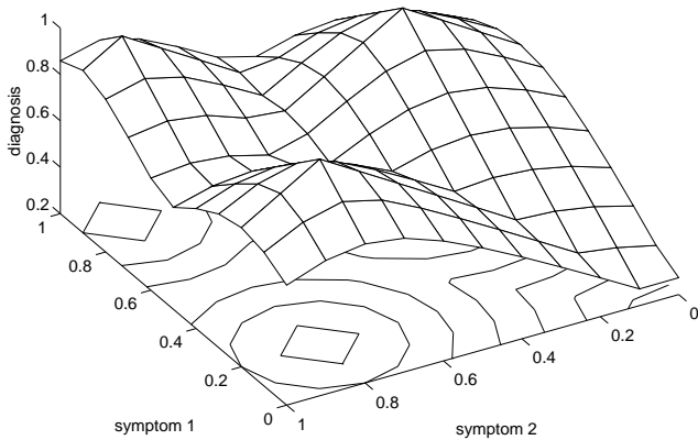
Fig. 5: Modeling of three faults with two symptoms using \gamma_C
