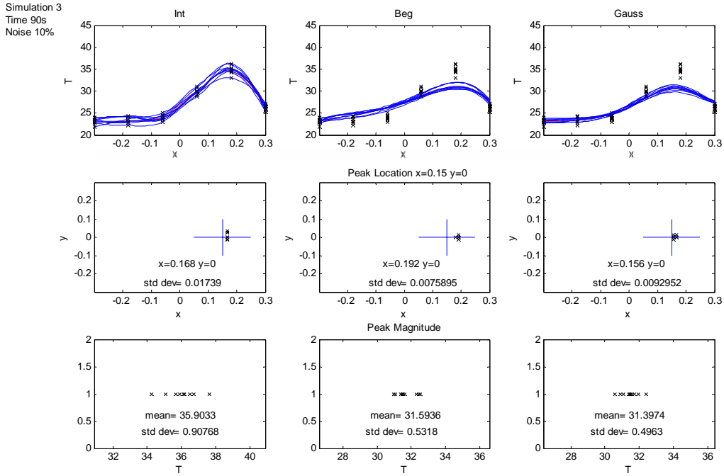
Fig. 3. Plots Format used to Compare the Algorithms
